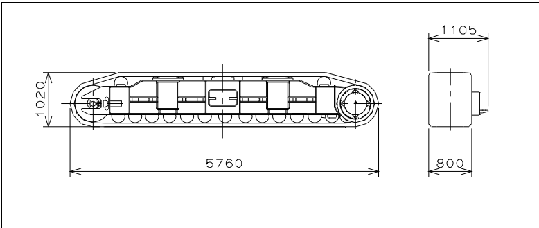
2) Crawler side frame 7.0 t x 2 pc
