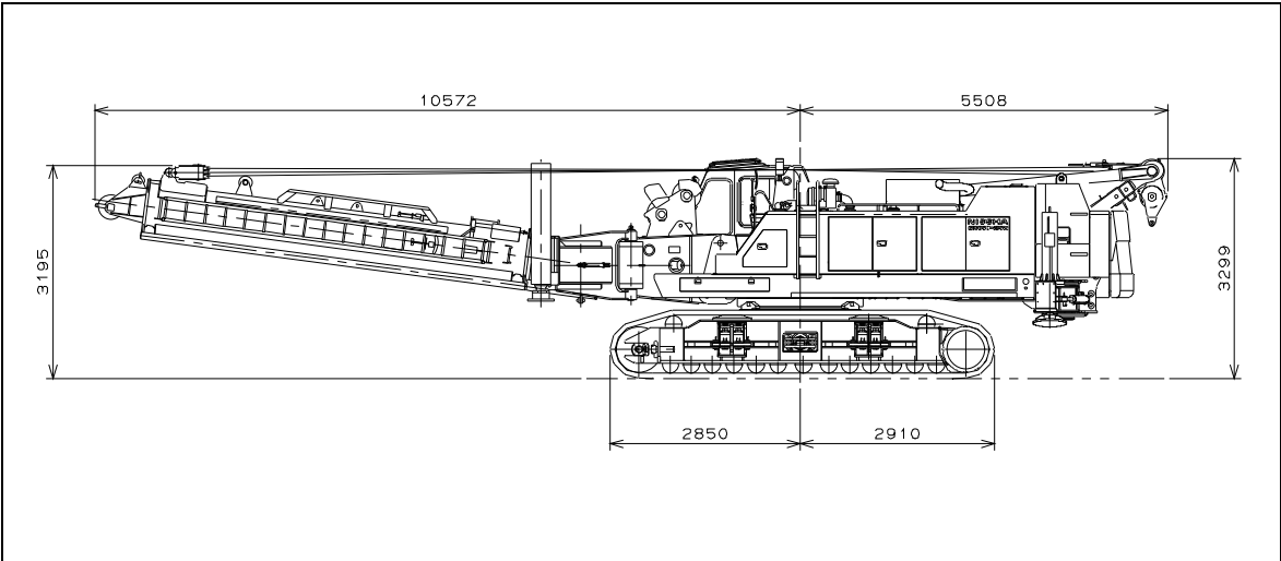
1) Superstructure 28.4 t (29.5 t with fourth drum option)
